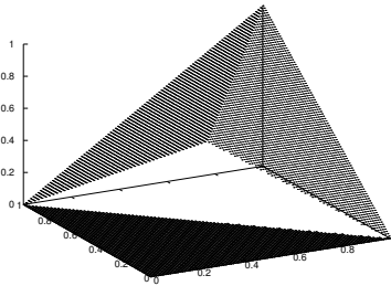
Figure 2.4: Nilpotent Minimum t-norm.
