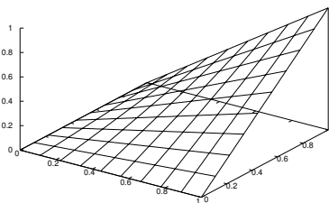
Figure 2.3: Product t-norm.
