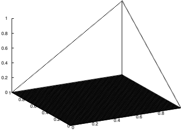
Figure 2.5: Drastic Product t-norm.
