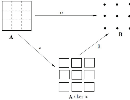
Figure A.1: First homomorphism theorem.
