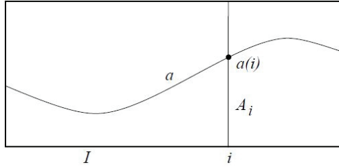
Figure A.2: Generalized direct product.
