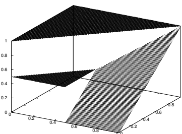
Figure 2.11: RDP residuum, a = \frac{1}{2} .
