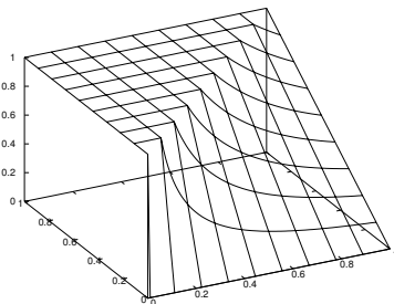
Figure 2.9: Product residuum.
