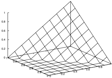
Figure 2.1: Łukasiewicz t-norm.
