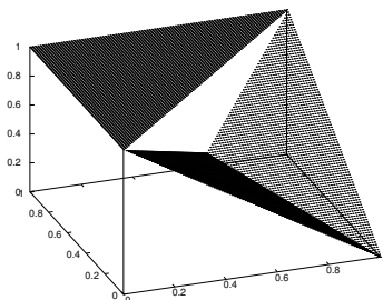
Figure 2.10: Nilpotent Minimum residuum.
