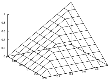
Figure 2.2: Gödel t-norm.
