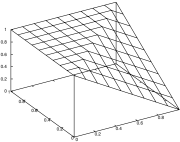
Figure 2.7: Łukasiewicz residuum.
