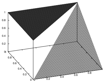
Figure 2.8: Gödel residuum.
