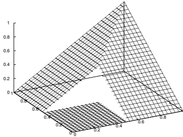
Figure 2.6: Revised Drastic Product t-norm: a = \frac{1}{2} .
